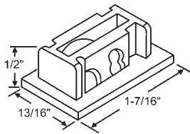
52-676 17/32" Dia. Metal Wheel
