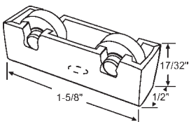
900-11791 Two 17/32" Dia. Metal Wheel
