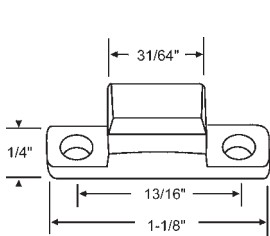
900-2003 Nylon Bottom Rail Slide Black
