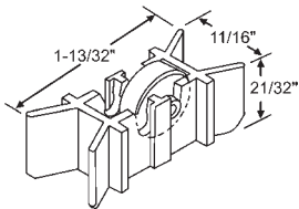
900-12993 17/32" Dia. Wheel
