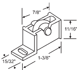
52-680 9/16" Dia. Nylon Wheel
