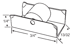
52-615 5/16" Dia. Nylon Wheel
