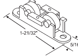
900-10419 Two 17/32" Dia. Nylon Wheels
