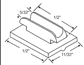
52-665 Insert for 52-667
