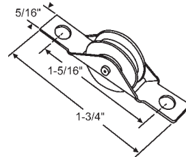
52-650 5/8" Dia. Nylon Wheel
