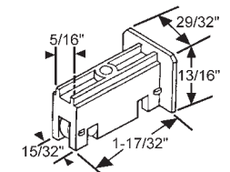
900-20286 17/32" Dia. Flat Ball Bearing Wheel w/Fixed Axle
