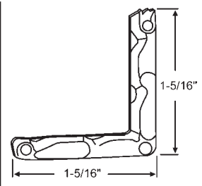
52-672 Slider Corner Key Die Cast
