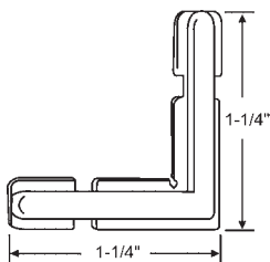
52-605 Slider Guide Angle Plastic
