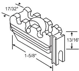
52-625 17/32" Dia. Metal Wheel
