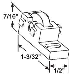
900-20289 17/32" Dia. Flat Metal Wheel w/ Separate Axle
