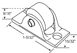
900-10027 29/64" Dia. Nylon Wheel with Die Cast Housing
