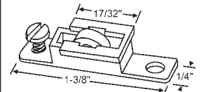
52-856 5/16" Dia. Flat Nylon Wheel White Acorn
