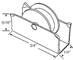
900-1276 5/16" Dia. Nylon Wheel
