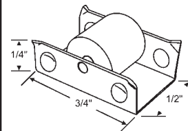
900-1278 11/32" Dia. x 3/8" Nylon Wheel
