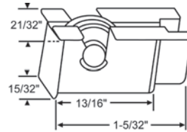
52-707 17/32" Dia. Metal Wheel
