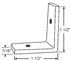
52-604 Slider Guide Angle Aluminum
