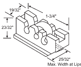
52-622 9/16" Dia. Metal Wheel
