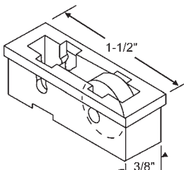
900-12609 17/32" Dia. Wheel Roller Projects 1/16" in Position "A" and 3/32" in Position "B".
