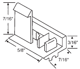
52-636 RH Storm Slider
