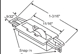
52-766 9/32" Dia. Metal Wheel
