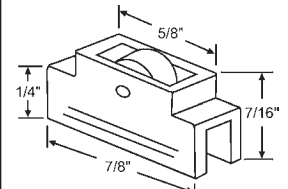
52-643 5/16" Dia. Metal Roller
