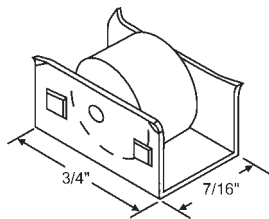
900-1285 15/32" Dia. Flat Nylon Wheel
