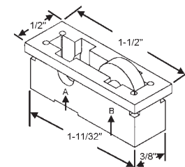
900-21376 17/32" Dia. Metal Wheel with Separate Axle. Roller Projects 1/32" in Position "A" and 1/8" in Position "B".
