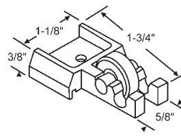
900-8512A 9/16" Dia. Flat Metal Wheel w/Separate Axle
