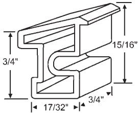
52-7000 Sash Lift Stop. Black Acorn
