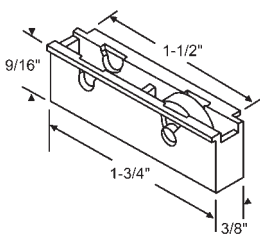
900-11564 17/32" Dia. Metal Wheel
