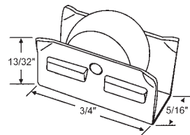
52-614 1/2" Dia. Nylon Wheel
