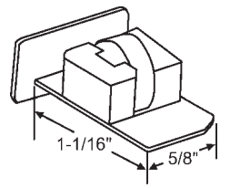
52-808 9/16" Dia. Flat Metal Wheel w/Separate Axle
