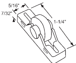
52-728 9/16" Dia. Steel Ball Bearing Wheel
