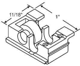
52-713 17/32" Dia. Flat Wheel
