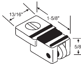
52-682 9/16" Dia. Metal Wheel with Die Cast Housing. Used with Plate 900-16252
