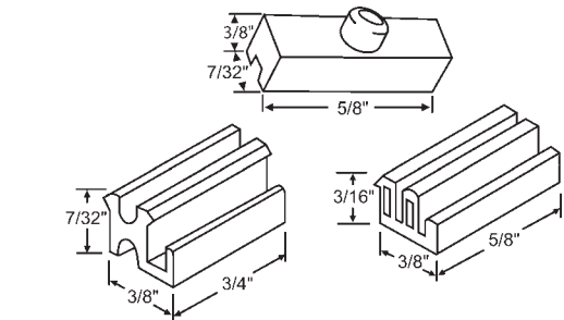
52-720 Repair Kit (2 of each) Alenco
