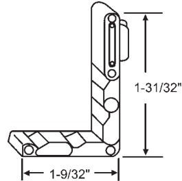
52-667 Slider Corner Key Die Cast with Plastic Insert Reynolds/Portalum
