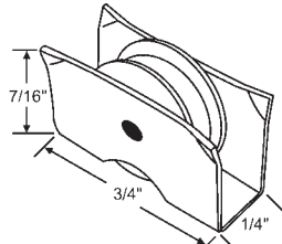
900-8374 5/16" Dia. Nylon Wheel
