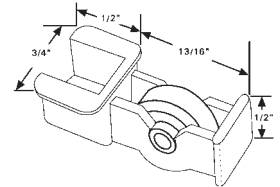
900-9765 17/32" Dia. Flat Ball Bearing Wheel w/Fixed Axle
