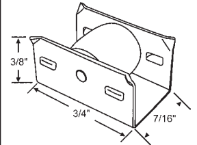
52-616 3/8" Dia. Nylon Wheel
