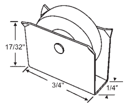
900-1290 5/8" Dia. Flat Nylon Wheel
