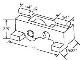
900-22 5/16" Dia. Flat Metal Wheel w/Fixed Axle
