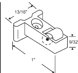
52-638 5/16" Dia. Metal Wheel
