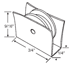
52-613 9/16" Nylon Wheel
