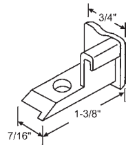
74-602A Set, 1 LH, 1 RH Airmaster
