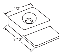
76-600 Uses Screw 20-004
