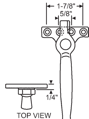
Use Screw 20-030
