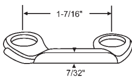
50-684 White Bronze
