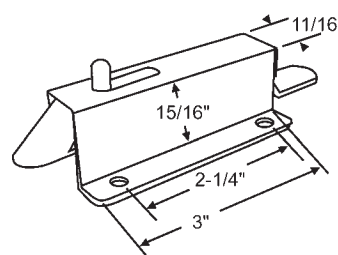
50-919 Aluminum
