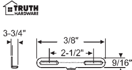
39-202 Stainless Steel
