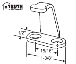
39-202 Stainless Steel
