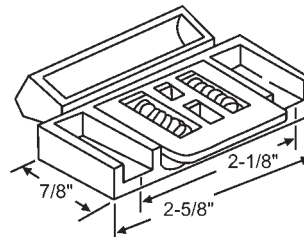
50-660 Nylon
