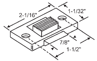
50-730 Black Plastic
