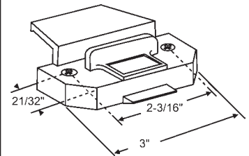
900-6734B Die Cast with Tabs on Bottom. Black Capitol
