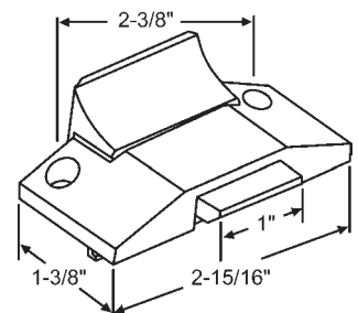
50-725 Black Aluminum
