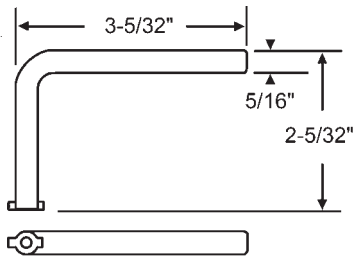
900-21413 Handle Cam Wrench with 1/8" Hex
