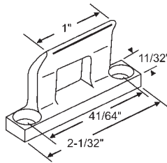
900-9107 Keeper for 32-277
