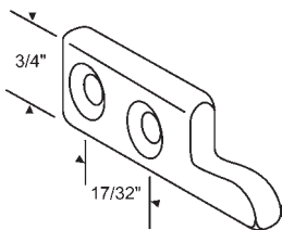
50-717 Brass
