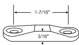
50-695 White Bronze
