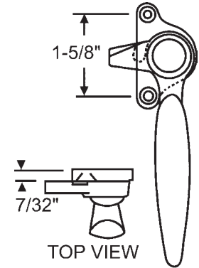
Water Rolled Finish Project Out Handle
