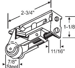
9-303 Flat Roller, Die Cast
