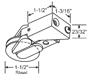
9-268 Die Cast Keller/Air Control
